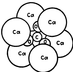
FIG. 1.—Arrangement of atoms in calcite, looking along the short diagonal of the rhombohedron. (Bragg.)
